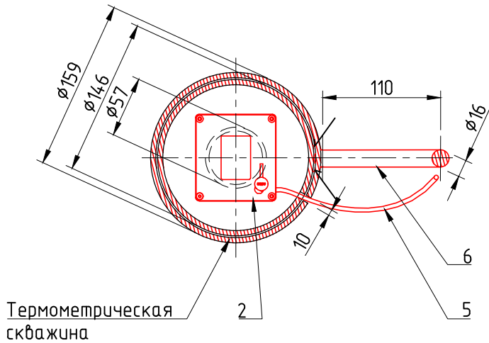
1-1 (1:5)
